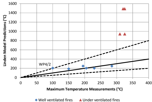
Figure 5. Comparison of maximum temperature measurements and Linden model predictions. Solid line indicates exact agreement between predictions and measurements, dashed lines indicate a factor of two difference.
