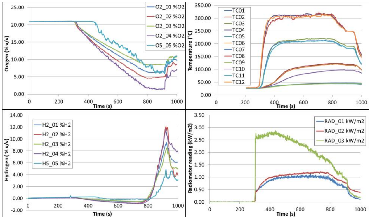
Figure 3. Oxygen, hydrogen, temperature and radiometer measurements from test WP4/10.
