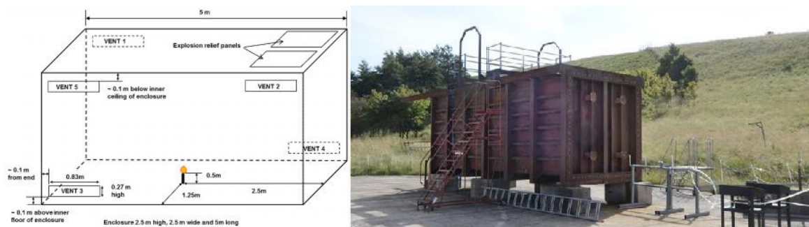
Figure 1. The HSL 31 m 3 enclosure
