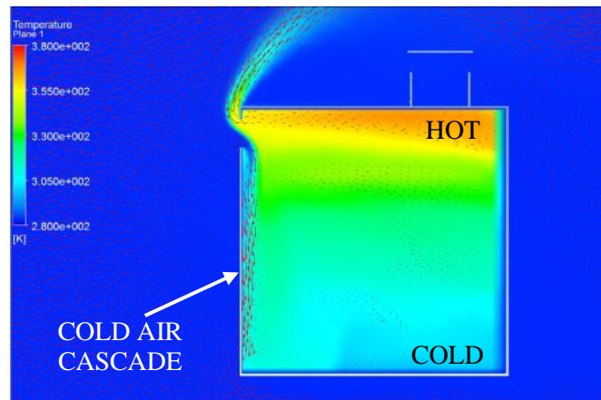
Figure 6 CFD model predictions of temperatures and velocities for experiment WP4-2 on a cross section through the enclosure.
