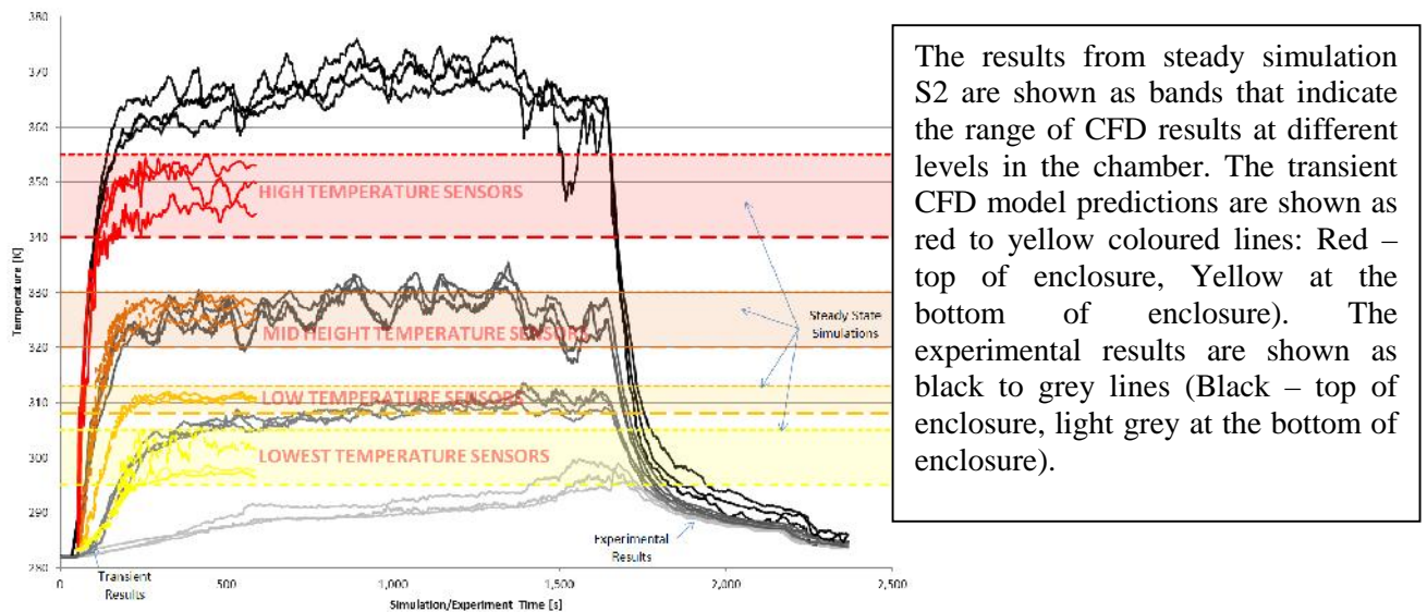
Figure 7 Comparison of CFD model temperature predictions and experimental measurements for experiment WP4-2.
