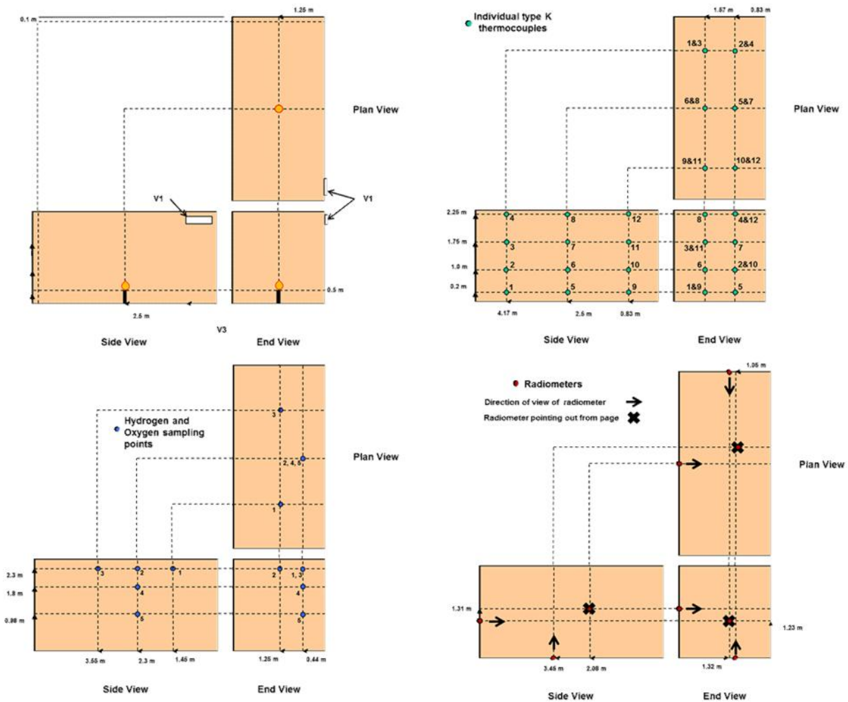
Figure 2. Positions of thermocouples, gas sampling points and radiometers relative to hydrogen flame and passive vent number 1
