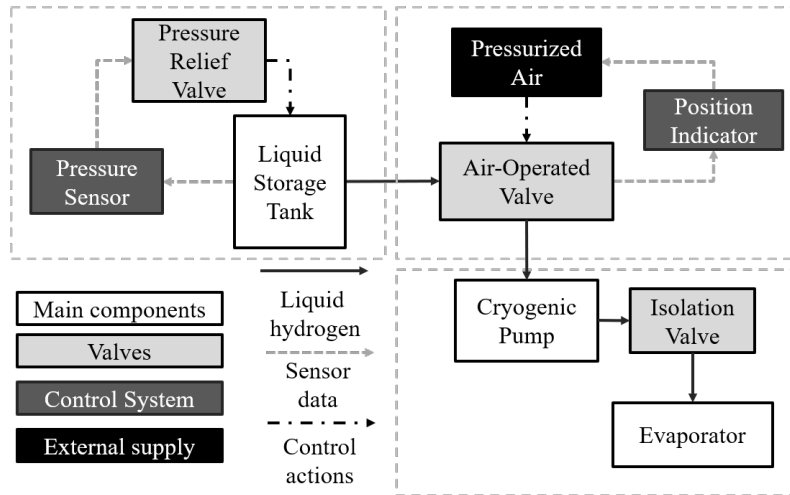
Figure 5: Liquid storage system case study block diagram.
