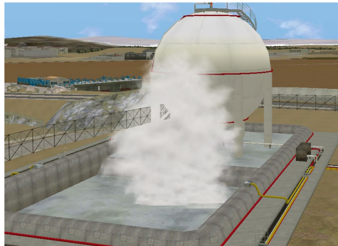
Figure 3. LH2 leak, dispersion, and possible pool formation at a storage facility.
